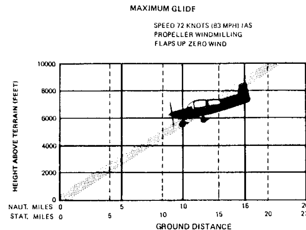
Figure 3.1 Maximum Glide
