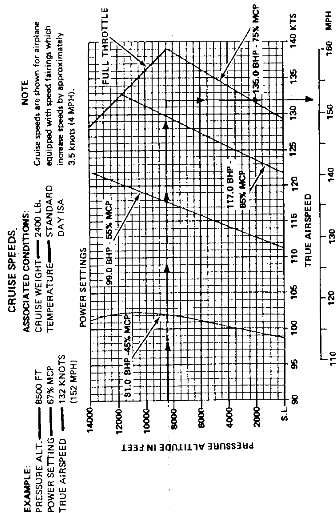
Figure 5-11. Cruise Speeds
