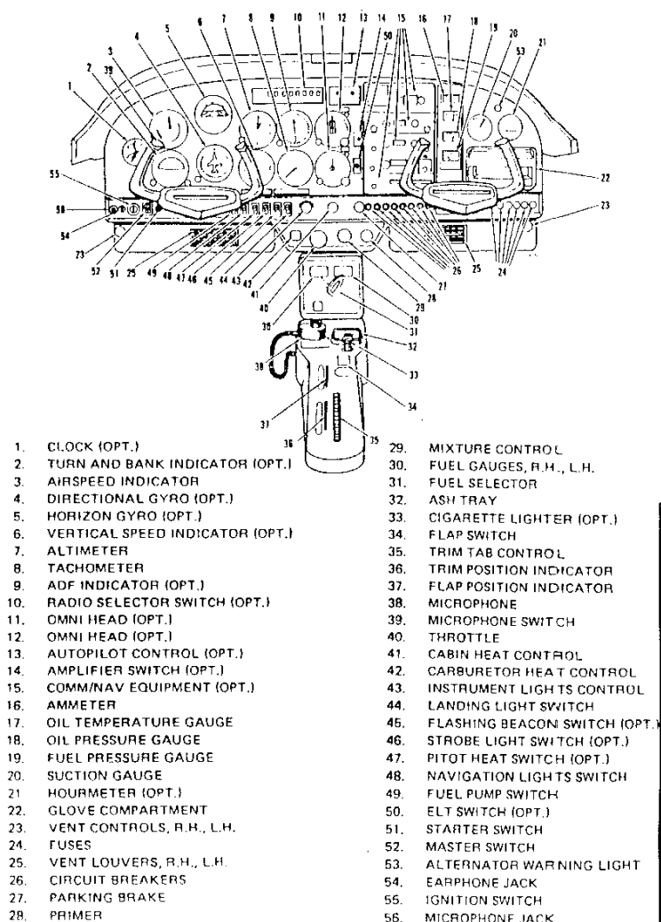
Figure 7-1. Instrument Panel
