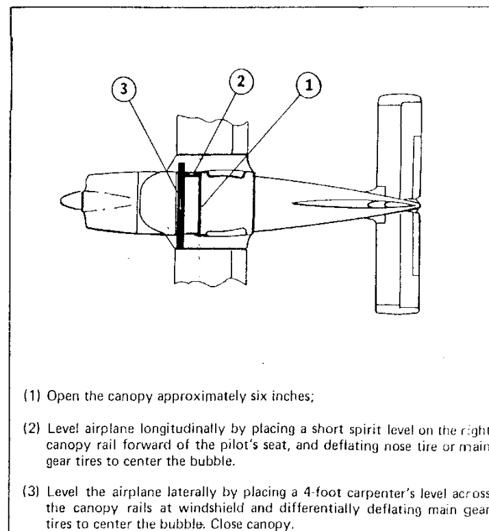
Figure 6-1. Airplane Leveling
