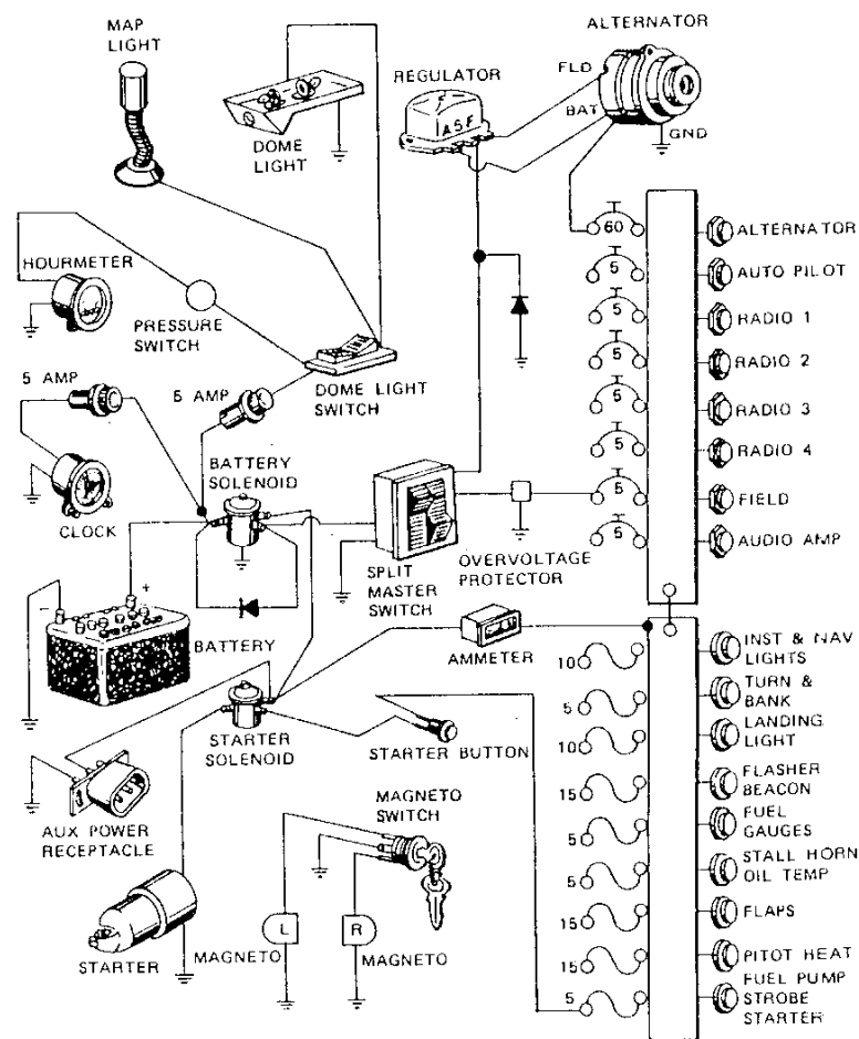
Figure 7-3, Electrical System
