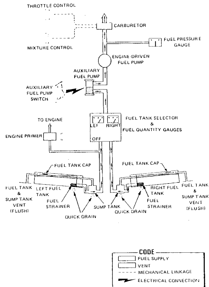
Figure 7-2 Fuel System
